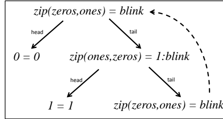
Fig. 1. Intuitive proof by circular coinduction of \text{zip}(\text{zeros}, \text{ones}) = \text{blink}
